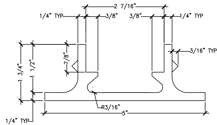
TRENCH DRAIN BODY
